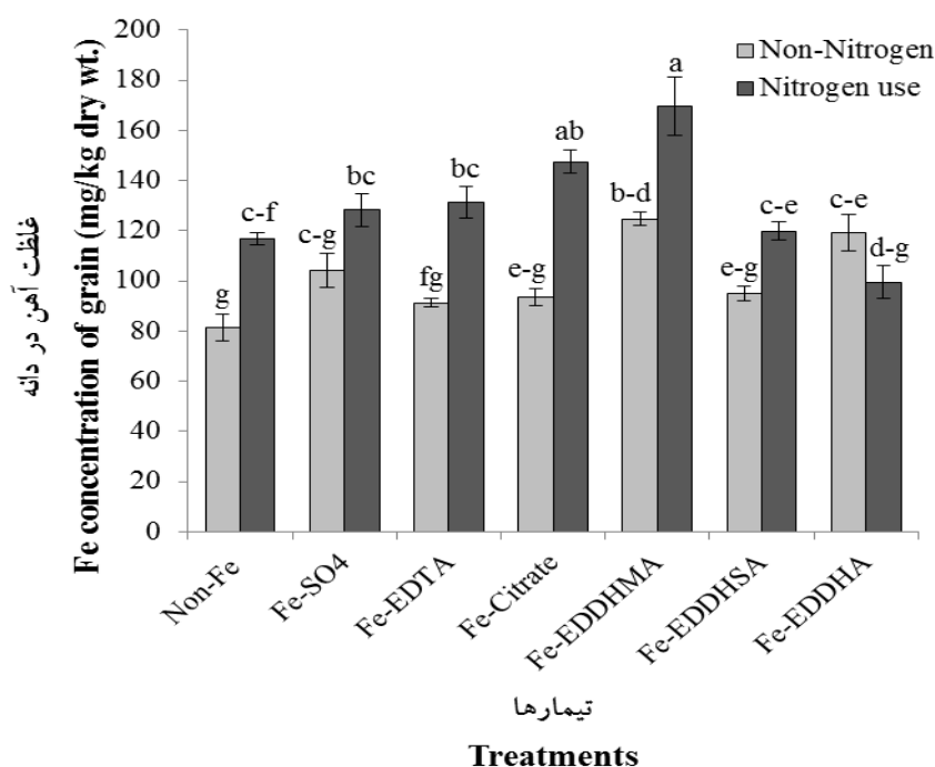
شکل ۱- مقایسه میانگین اثر متقابل کاربرد آهن و نیتروژن بر غلظت آهن در دانه گندم Figure 1- Mean comparison of interactions between iron and nitrogen application on Fe concentration of grain wheat (Means in each column followed by similar letters are not significantly different at the %5 probability level (LSD Test))
