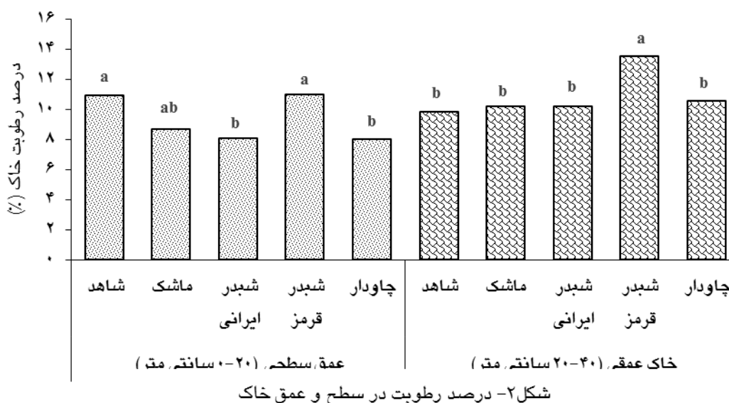
Figure 2. Soil moisture percent in surface and deep soil
